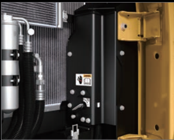
Battery Disconnect Switch with DEF Purge Notification Buzzer
